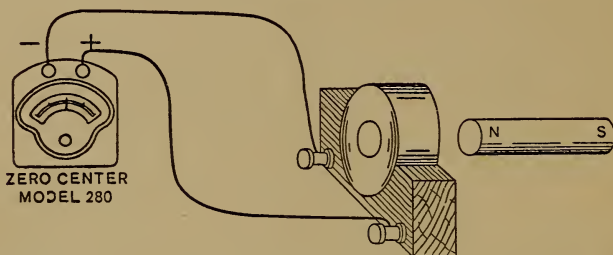
FIG. 8.—CURRENT INDUCED BY MAGNETISM. Turner's Method.
